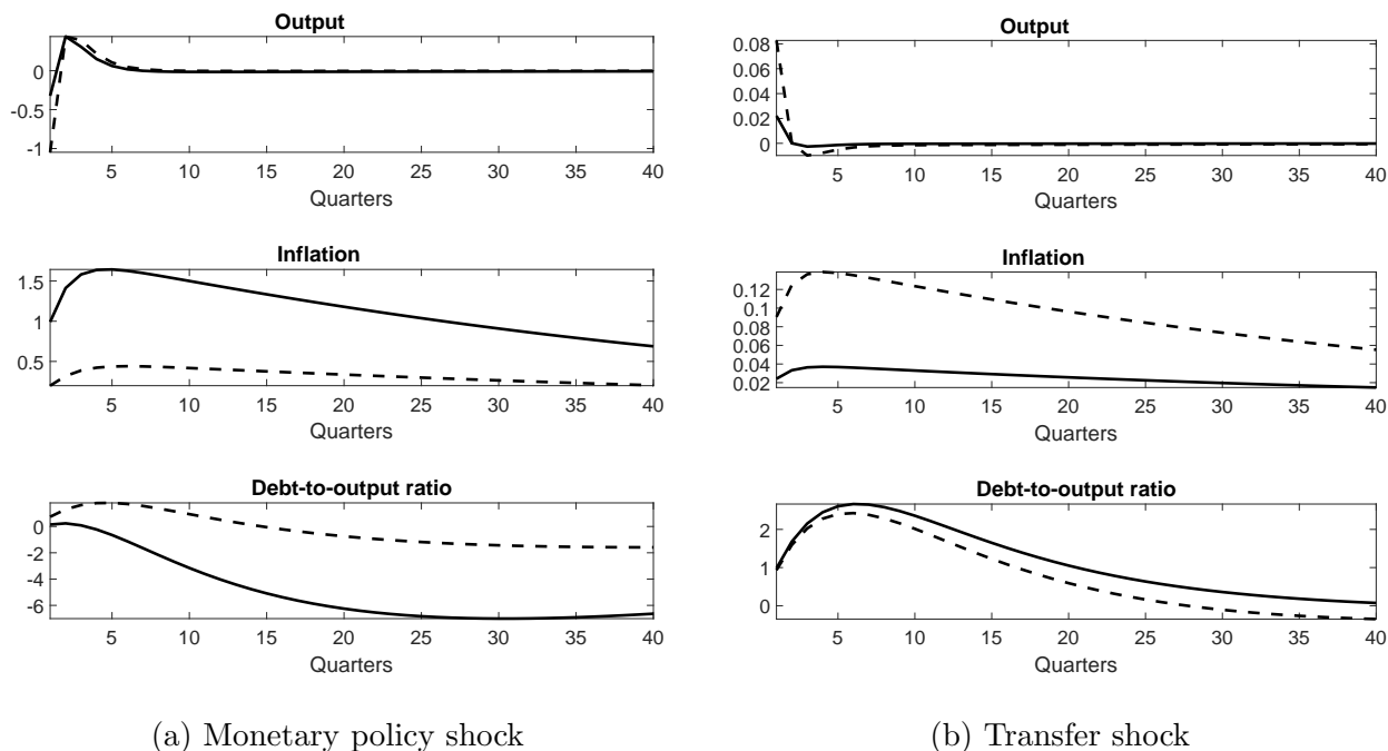
Figure 11: Impulse response functions to a contractionary monetary policy and a positive transfer shock in the indeterminacy regime. The bold line depicts the response in the indeterminacy regime (identical to Figure 10) as a reference. The dashed line shows how the transmission mechanism changes when all elements in M are set to zero. The unit of the impulse responses is percentage deviations from the steady state for output and percentage point deviations from the steady state for inflation and the debt-to-output ratio.
